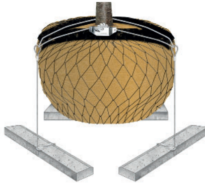
Tree Anchoring System: RF3RDMP
